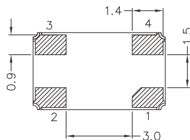
DIMENSION (mm)
