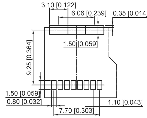
RECOMMENED P.C.B LAYOUT(TOP VIEW) GENERAL TOLERANCE ±0.05
