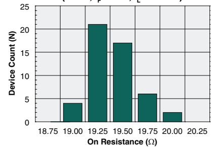
Typical On-Resistance Distribution (N=50, I_F=5\text{mA} , I_L=120\text{mA} )
