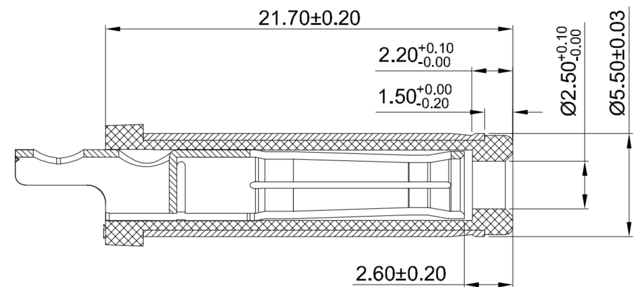
MATING PLUG \varnothing 5.5 \times 2.5 \text{mm}
