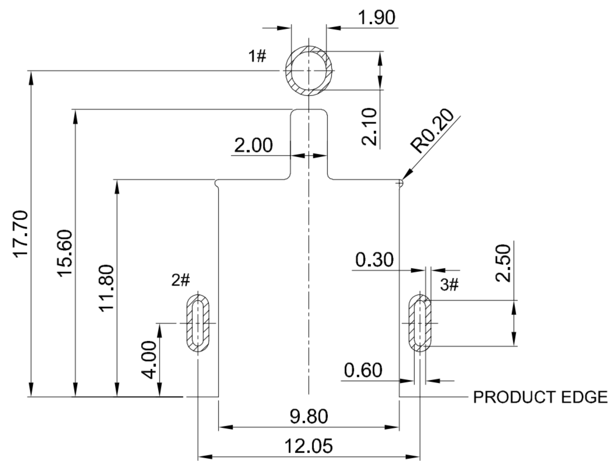
RECOMMENDED PCB LAYOUT TOLERANCE: \pm 0.05
