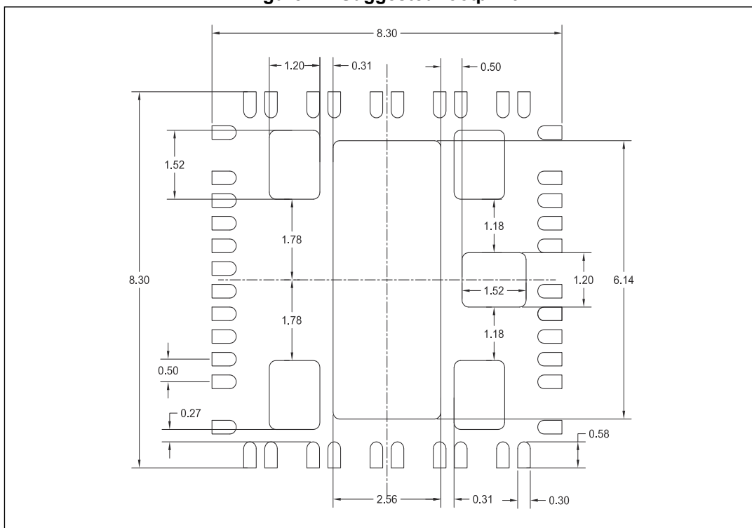
Figure 17. Suggested footprint
