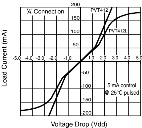
Figure 3. Linearity Characteristics
