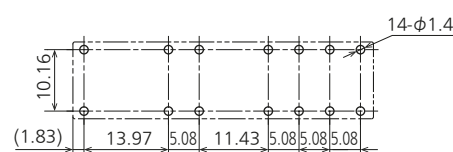
Recommended PC board pattern ( BOTTOM VIEW )
