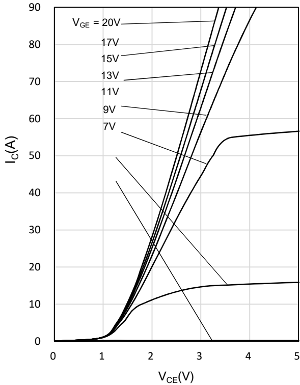
Fig. 1 Output characteristics
