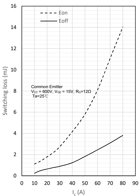
Fig. 8 Switching loss vs. collector current
