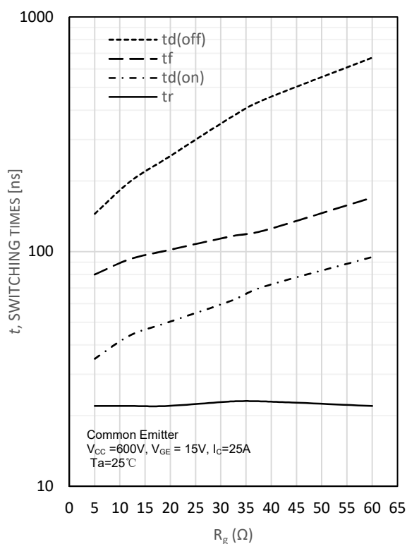
Fig. 5 Switching times vs. gate resistor
