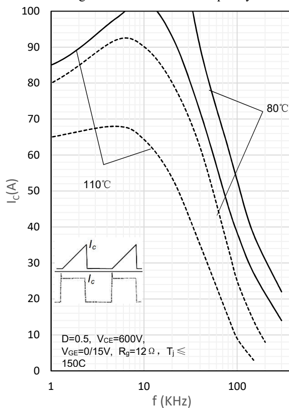
Fig. 2 Load Current vs. Frequency
