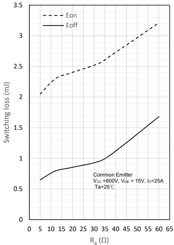
Fig. 7 Switching loss vs. gate resistor
