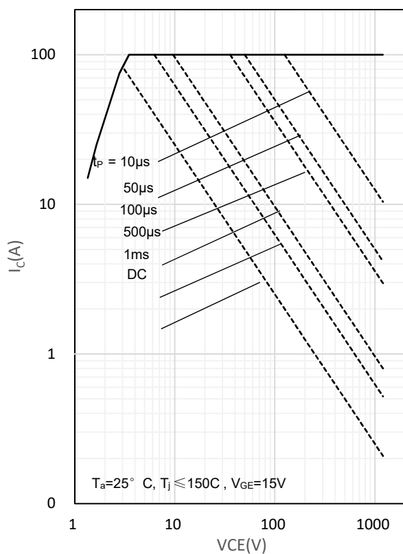
Fig. 1 FBSOA characteristics
