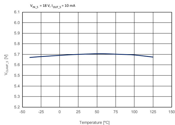
Figure 14. 5 V eFuse voltage clamp vs. temperature
