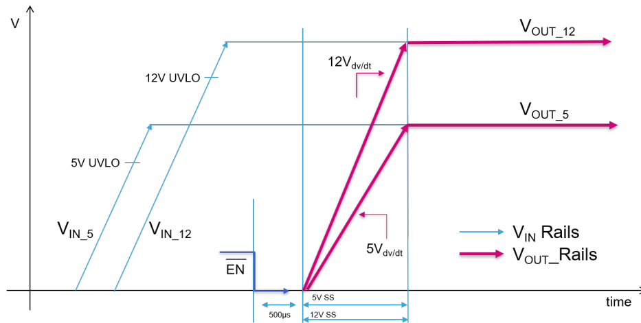
Figure 4. Typical start-up sequence (Enable after V_{IN} rise)
