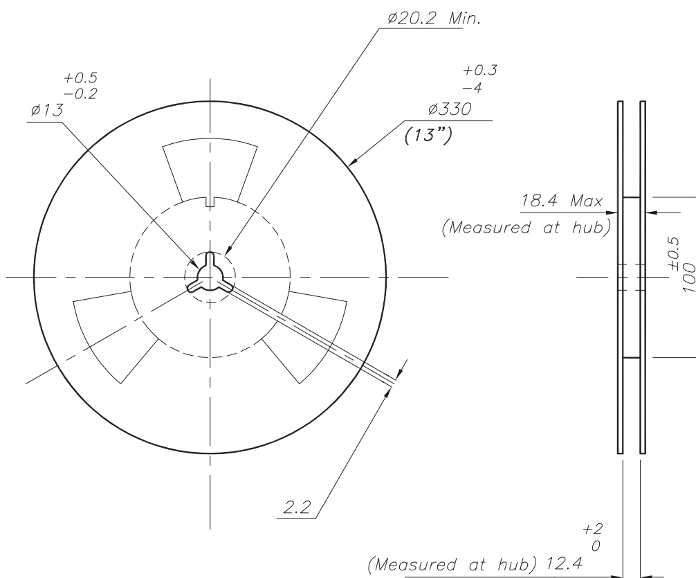
Figure 47. Reel drawing
