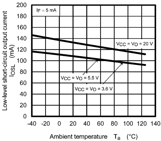
Fig. 12.2.9 I_{OSL} - T_a
