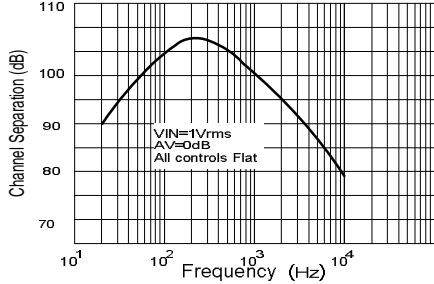
Fig.9 Channel Separation(L→R) vs. Frequency
