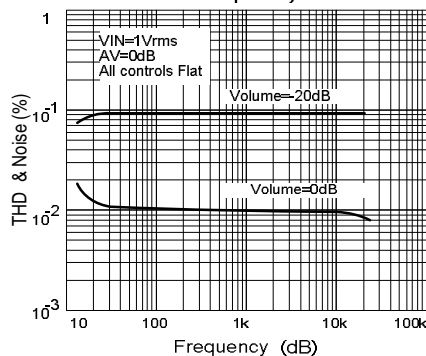
Fig.6 Distortion & Noise vs. Frequency
