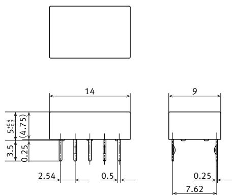
PC board terminal (self-clinching terminal)
