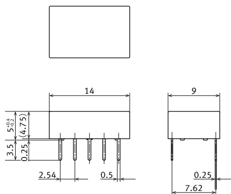
External dimensions PC board terminal (standard)
